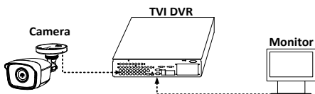
Figure 2-1 Connection
